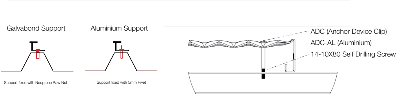
Detail B - channel to roof sheet
